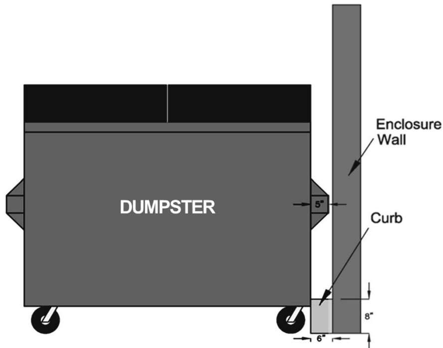
Figure 3: Curb Detail
