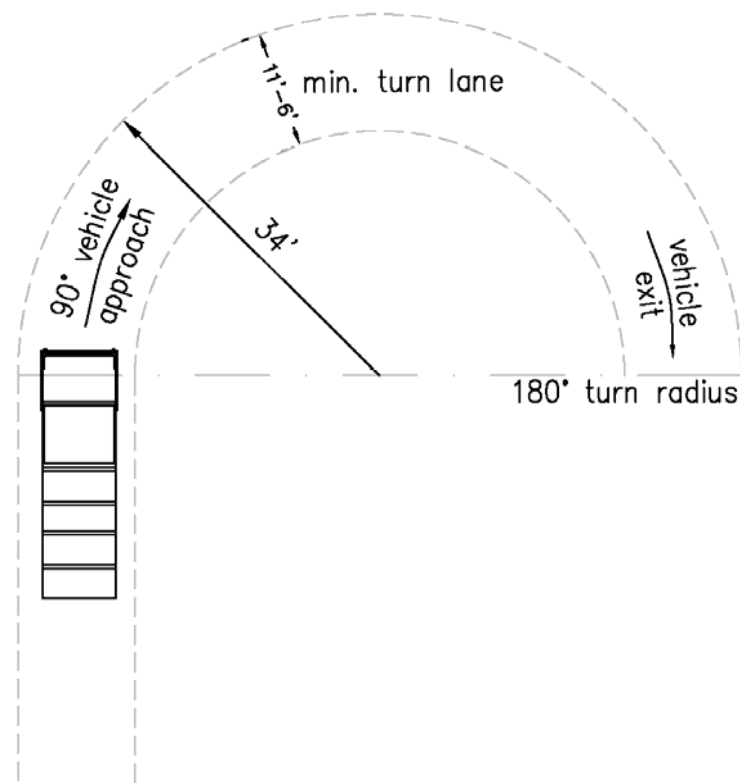
Figure 2: Truck Turning Radius
