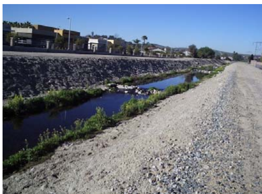
Figure 5-22. Rock Check Dam and Shallow Pools in CCCH
